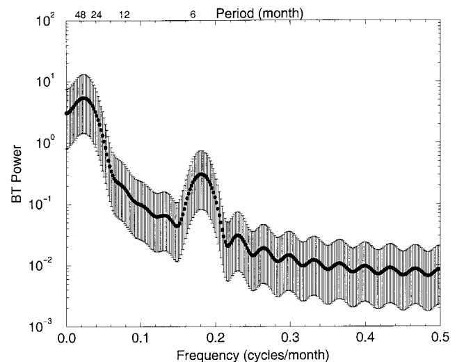
Figure 10. Blackman-Tukey correlogram estimate of the SSA-filtered SOI. The embedding dimension for SSA is M = 60 , and RCs 1–4 and 10–11 were chosen as most significant. A Bartlett window of width m = 30 was used for the spectral estimate of the prefiltered SOI. The error bars are based on a chi-square test and reach from the 2.5% to the 97.5% quantile.
